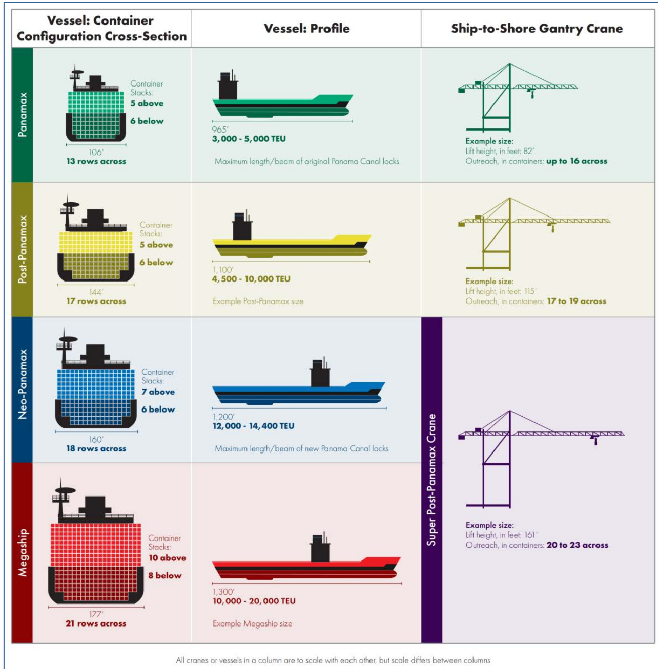
Figure 2-1: Increasing Vessel Size and its Impact on Port Infrastructure
