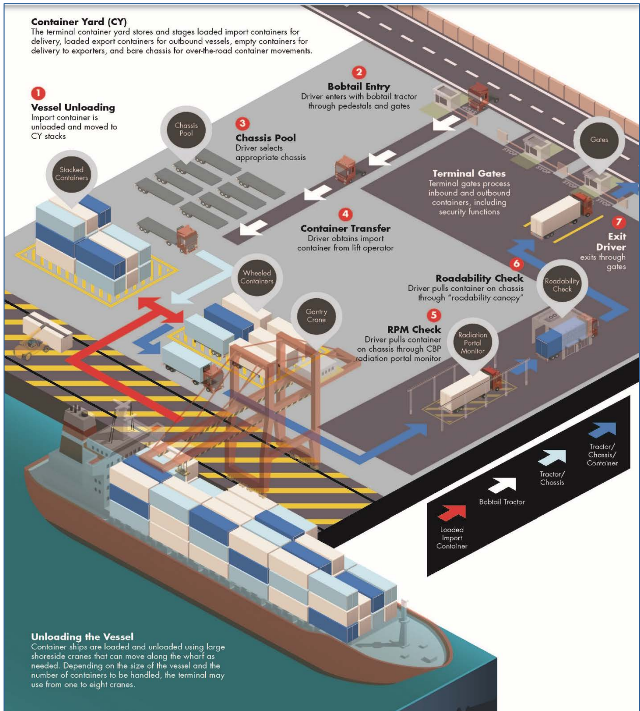
Figure C-1: Example of Container Terminal Flow
