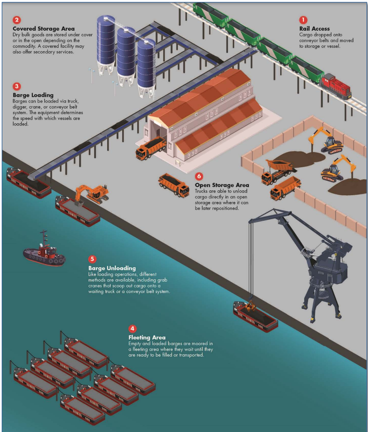
Figure C-2: Example of Dry Bulk Terminal Flow
