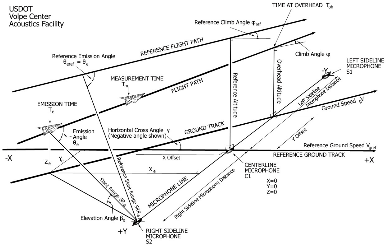
Figure 1 - Aircraft and Microphone Geometry
