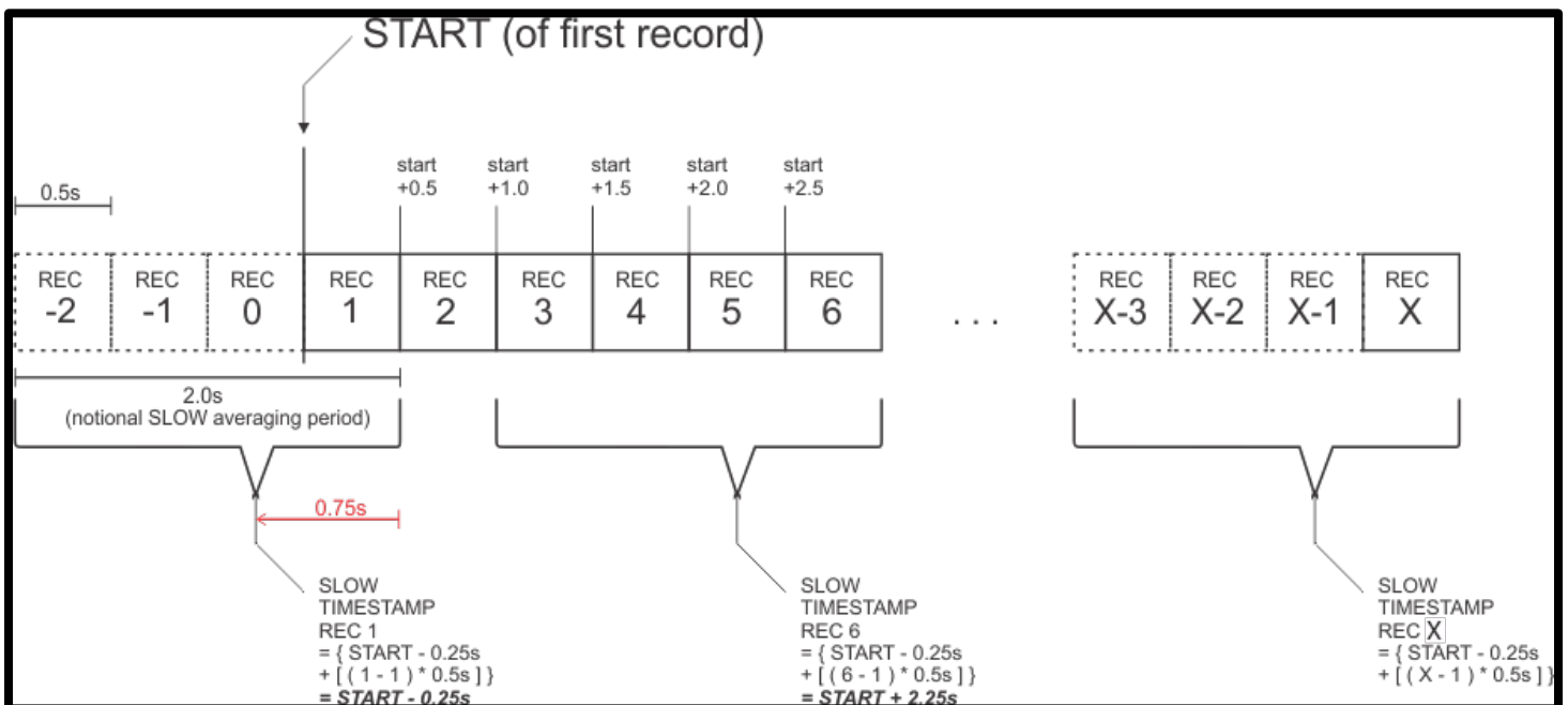
Figure 2 - Illustration of Start Times and Timestamps for Slow-Averaged Records
