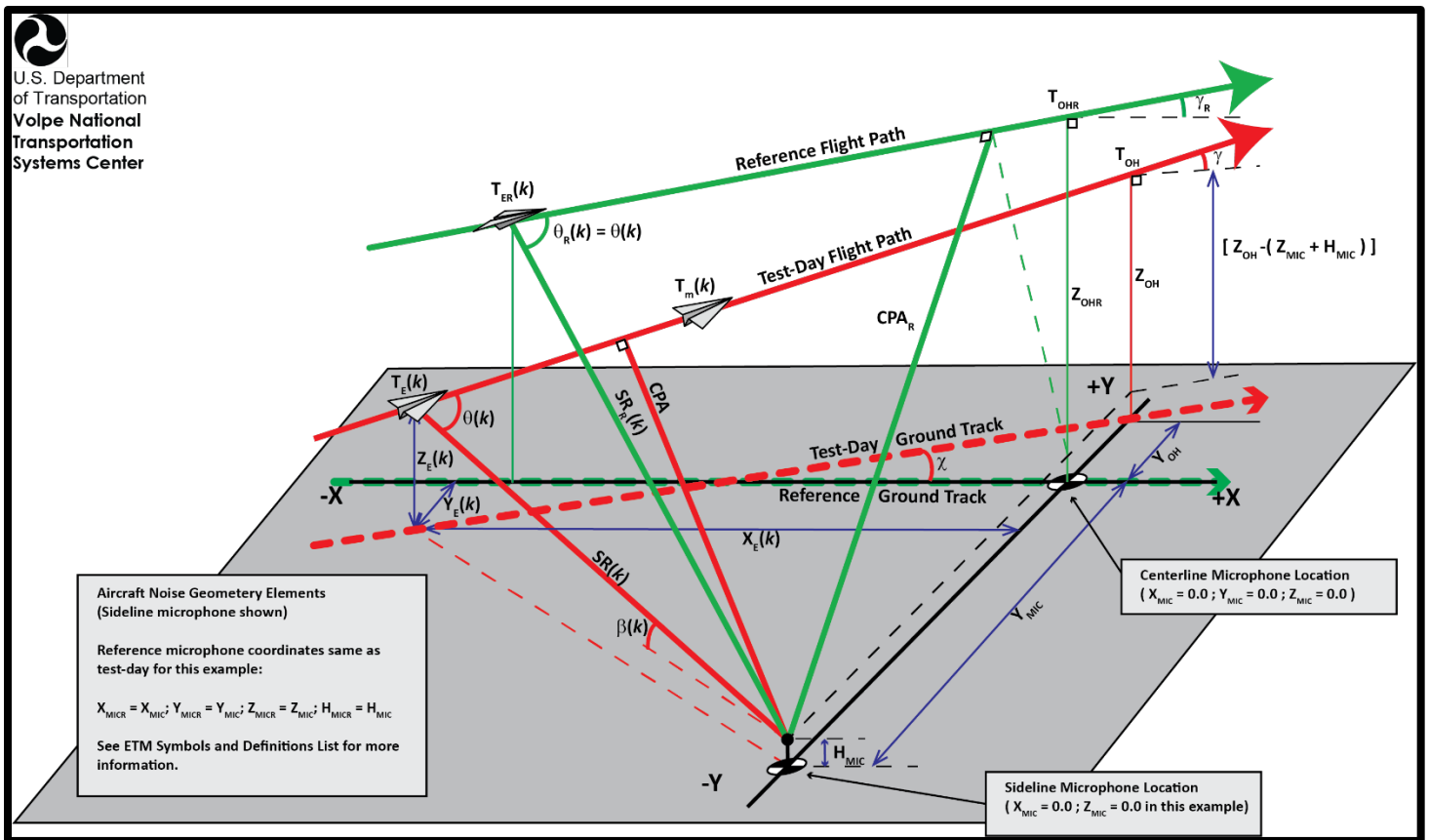
Figure 1 - Illustration of Noise Geometry for Test-Day and Reference Flight Tracks
