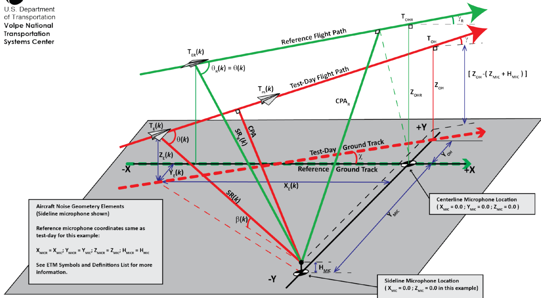
Figure 1- Example Aircraft Noise Geometry Elements
